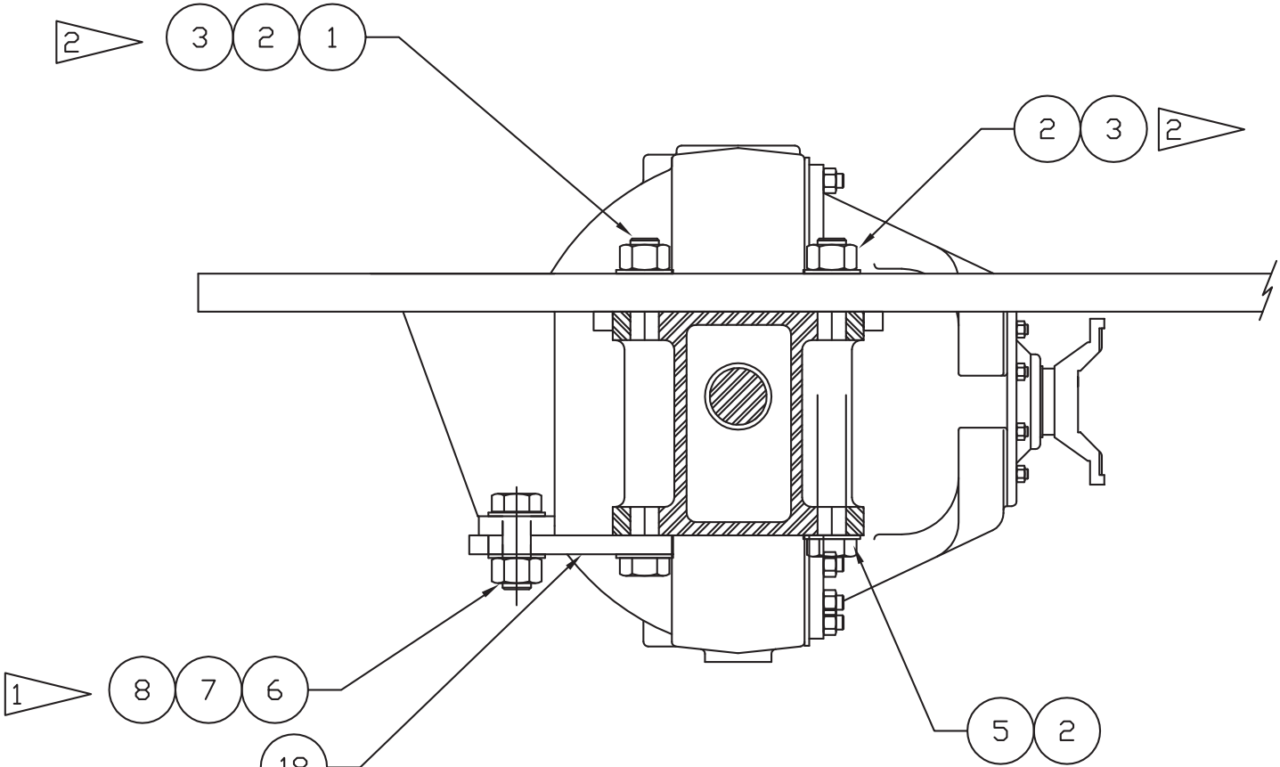
SECTION A-A BOGIE AXLE TORQUE REACTION LINK
