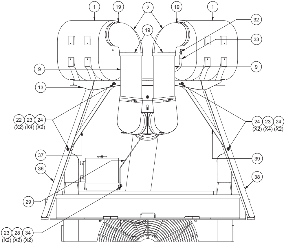
SECTION B-B
