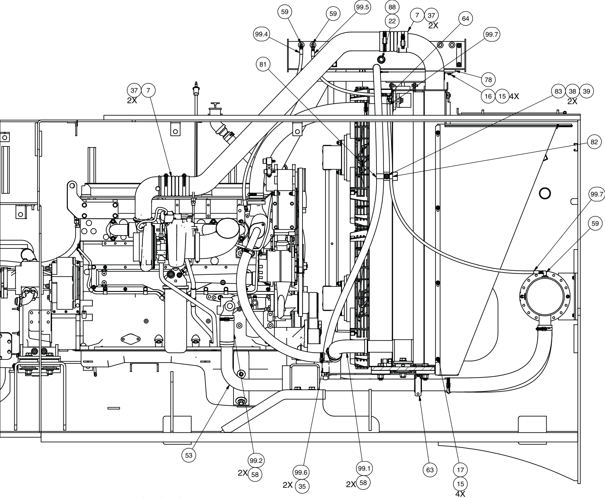
SECTION 2A-2A ITEMS REMOVED FOR CLARITY
