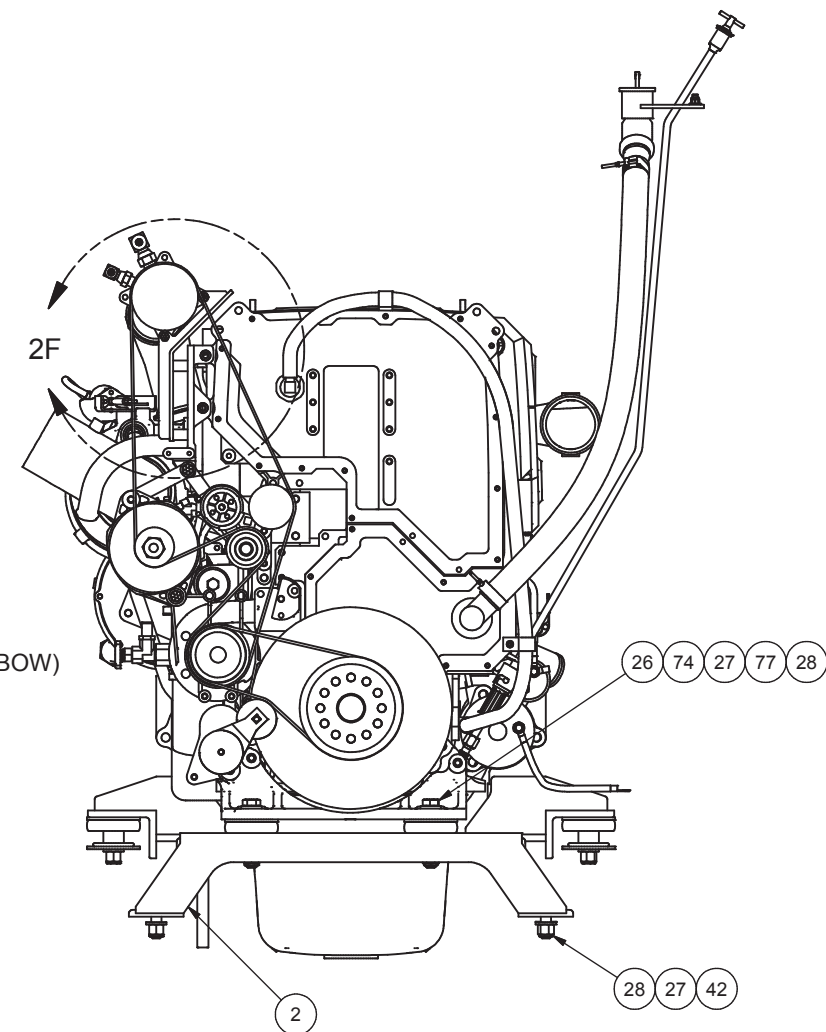
DETAIL 2F
