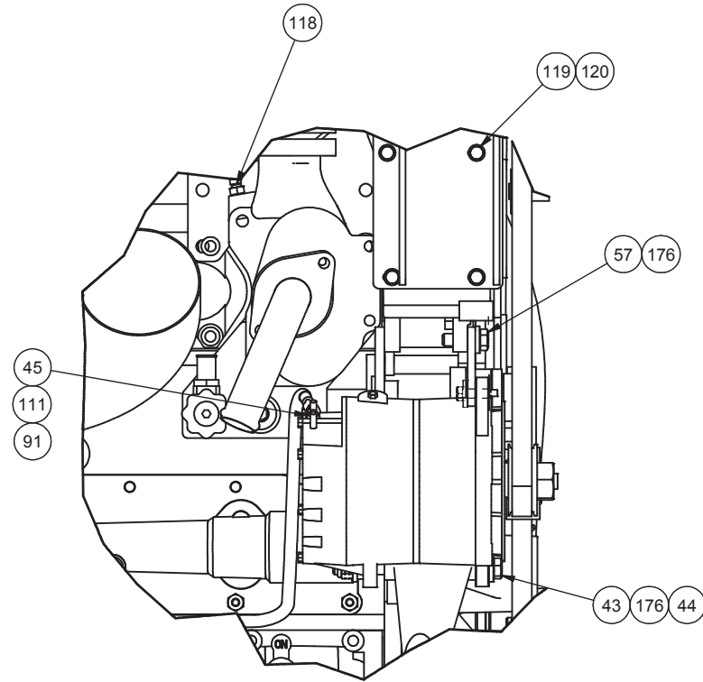
DETAIL 2B
