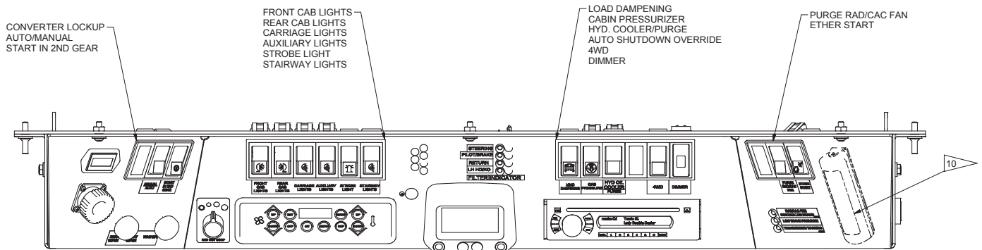
AUTOMATIC TRANSMISSION CONSOLE L60 LAYOUT
