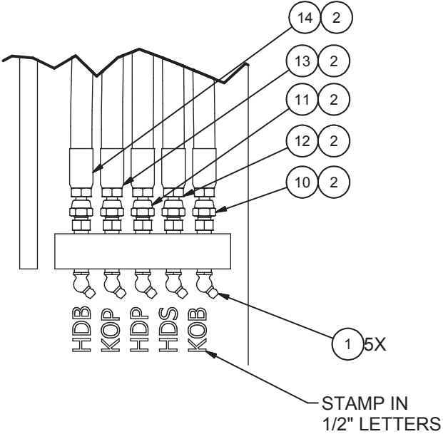
DETAIL B RIGHT SIDE GREASE BLOCK
