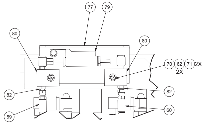
DETAIL 3D
