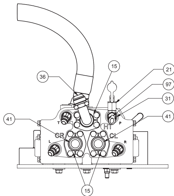
DETAIL C STEERING FLOW AMP
