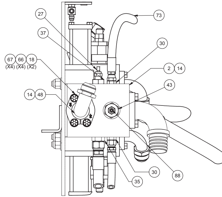
DETAIL E DUMP VALVE
