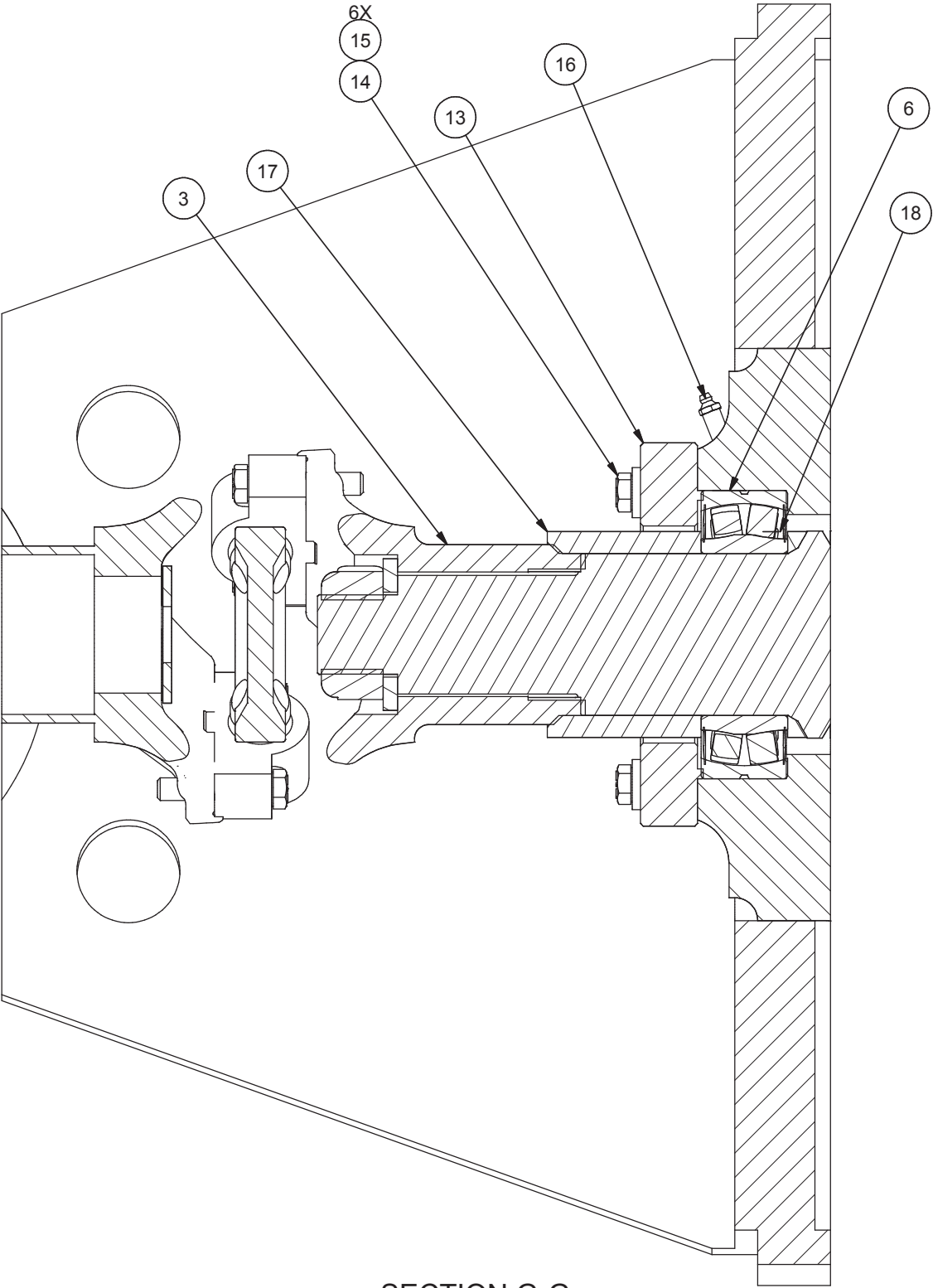
SECTION G-G
