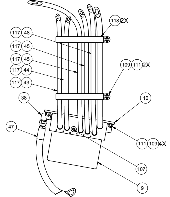
SECTION 3G-3G
