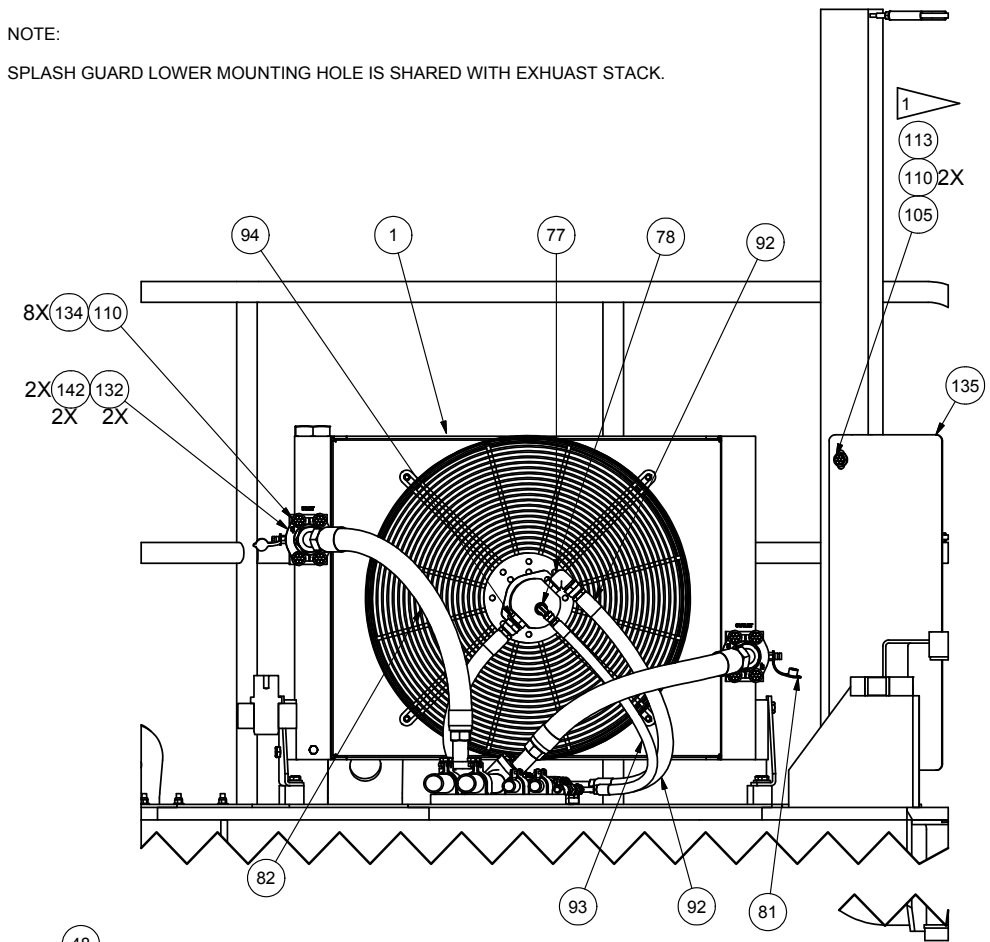
SECTION 3F-3F PARTS REMOVED FOR CLARITY
