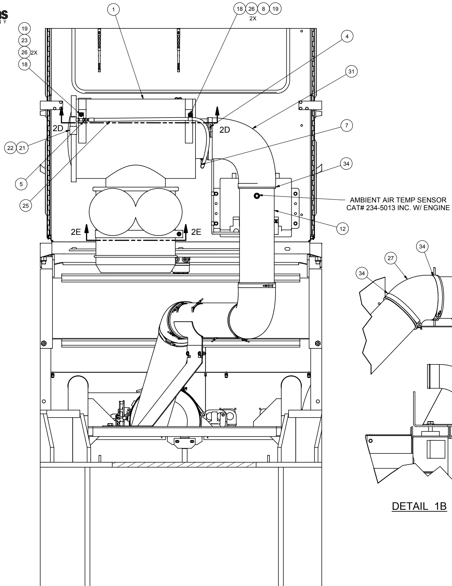
SECTION 1A-1A
