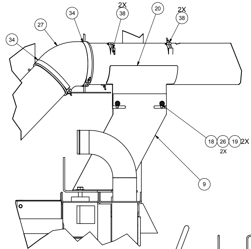
DETAIL 1B
