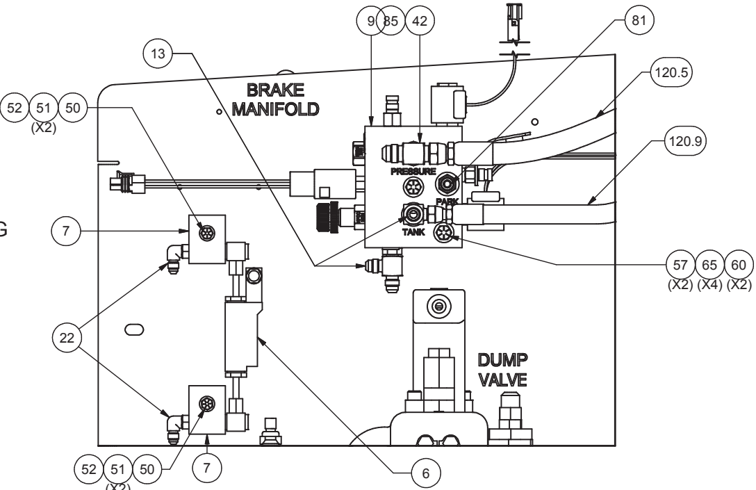
DETAIL B BRAKE MANIFOLD
