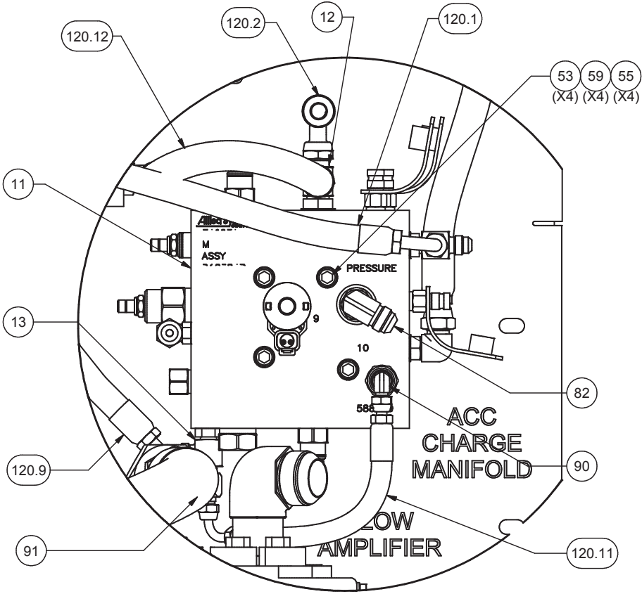
DETAIL G ACC CHARGE MANIFOLD
