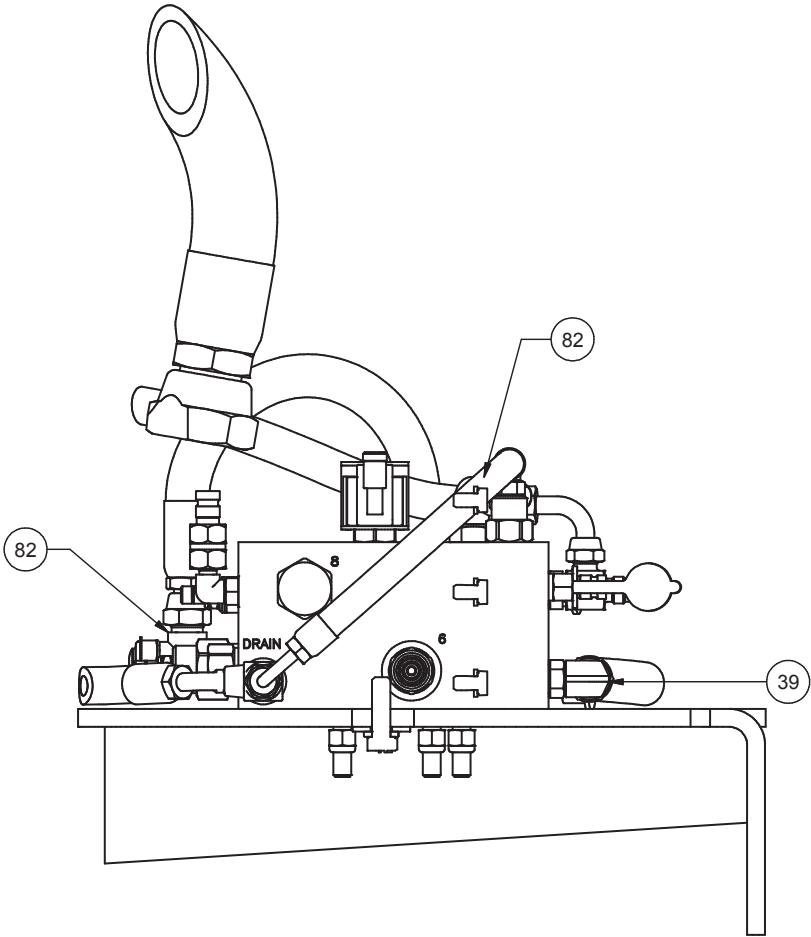
DETAIL G ACC CHARGE MANIFOLD
