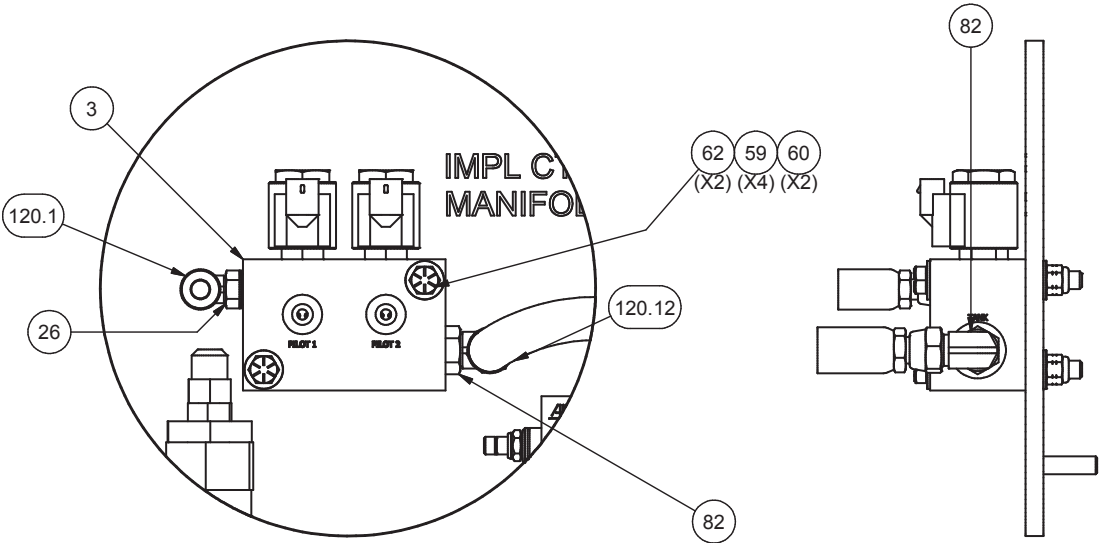
DETAIL H IMPLEMENT CONTROL MANIFOLD
