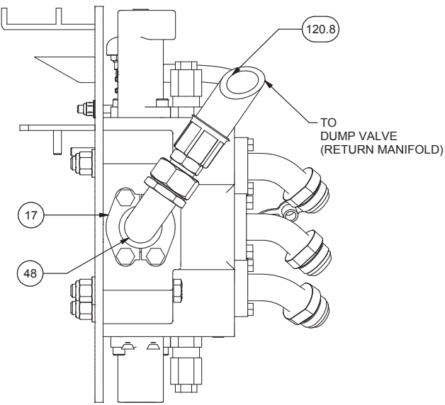
DETAIL D HOIST VALVE
