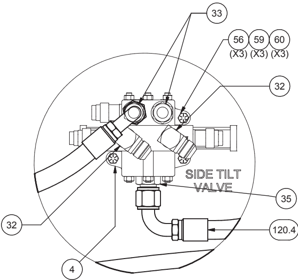
DETAIL A SIDE TILT VALVE
