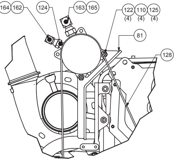
DETAIL D
