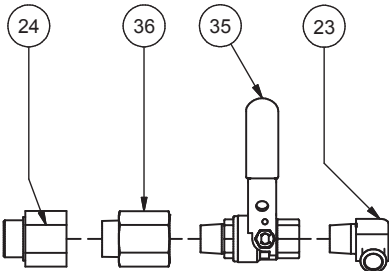
HEATER SUPPLY (DETAIL E; "HEATER RETURN", SIMILAR)
