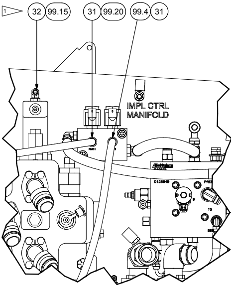
DETAIL F
