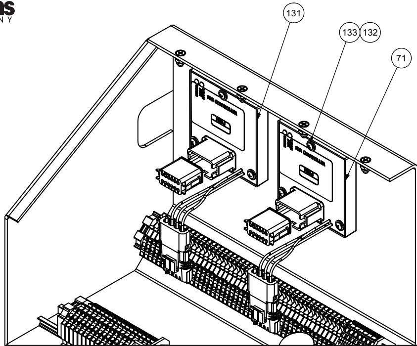
VIEW 3F3
