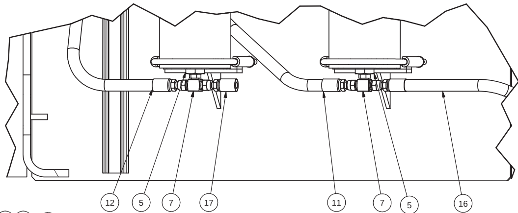
DETAIL D
