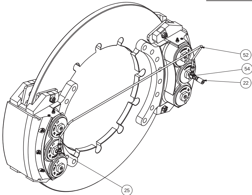
DETAIL F
