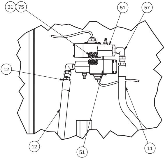
DETAIL E
