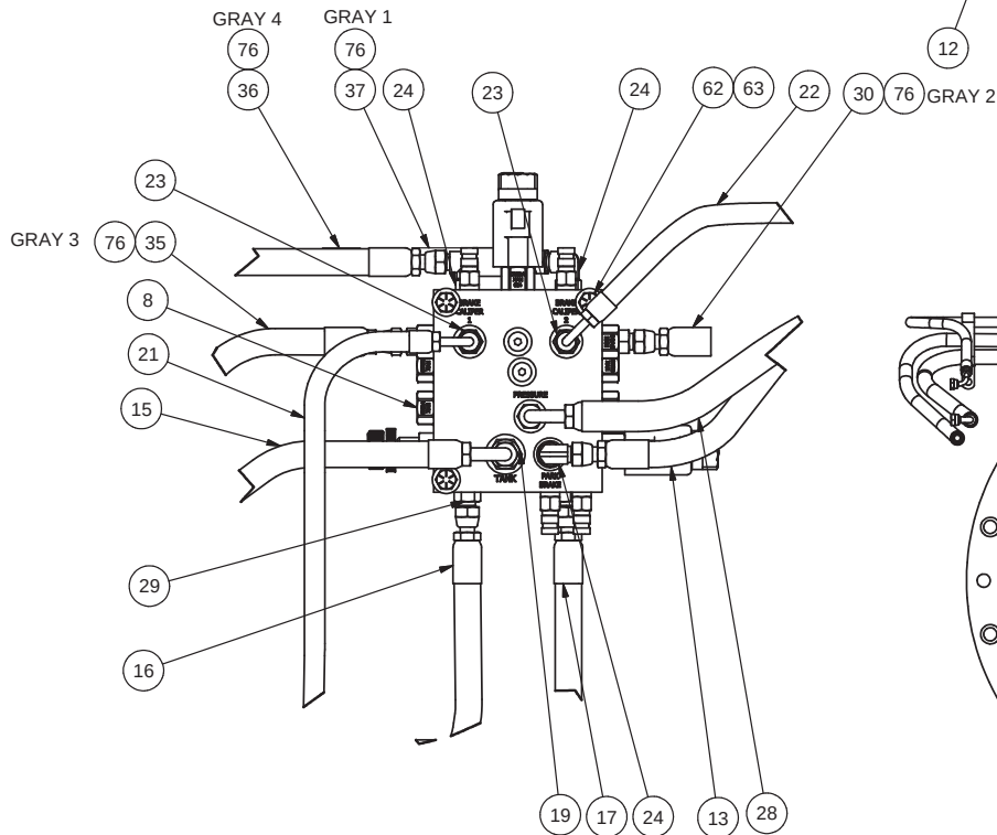
DETAIL F
