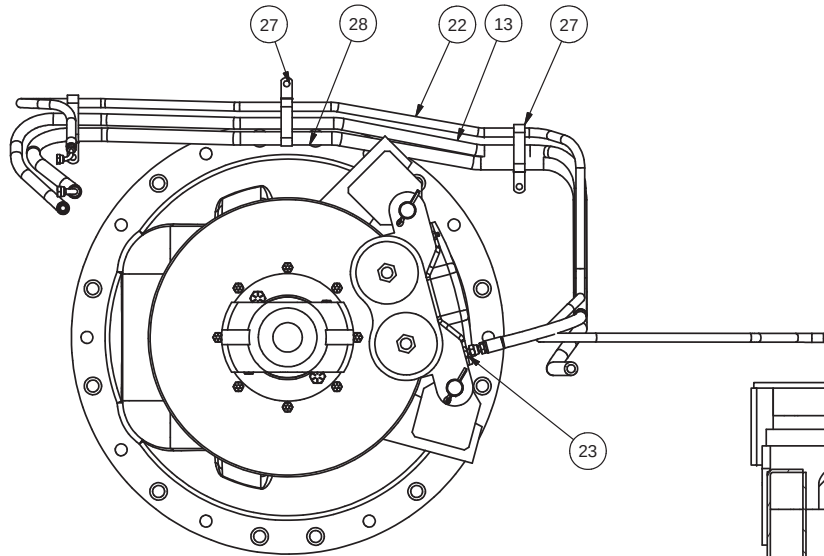
SECTION G-G
