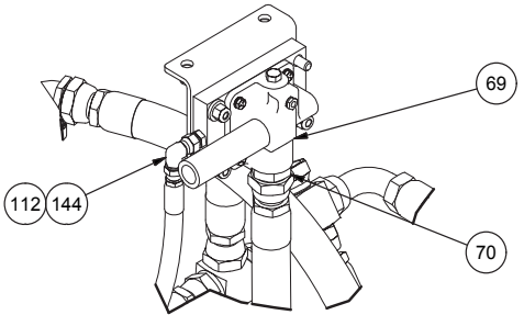
DETAIL 3K
