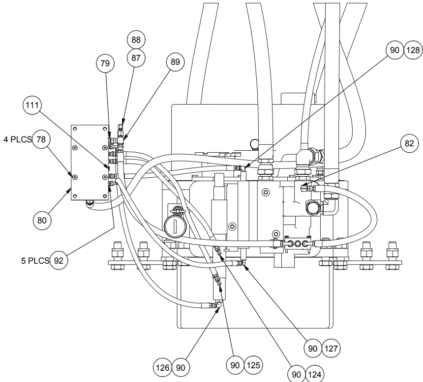
VIEW 3B-3B
