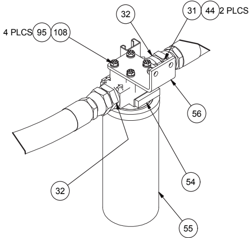
DETAIL 3D
