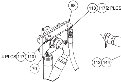
DETAIL 3J
