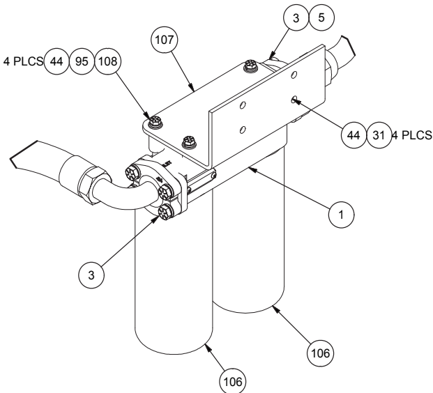
DETAIL 3G
