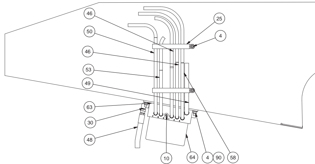
SECTION G-G
