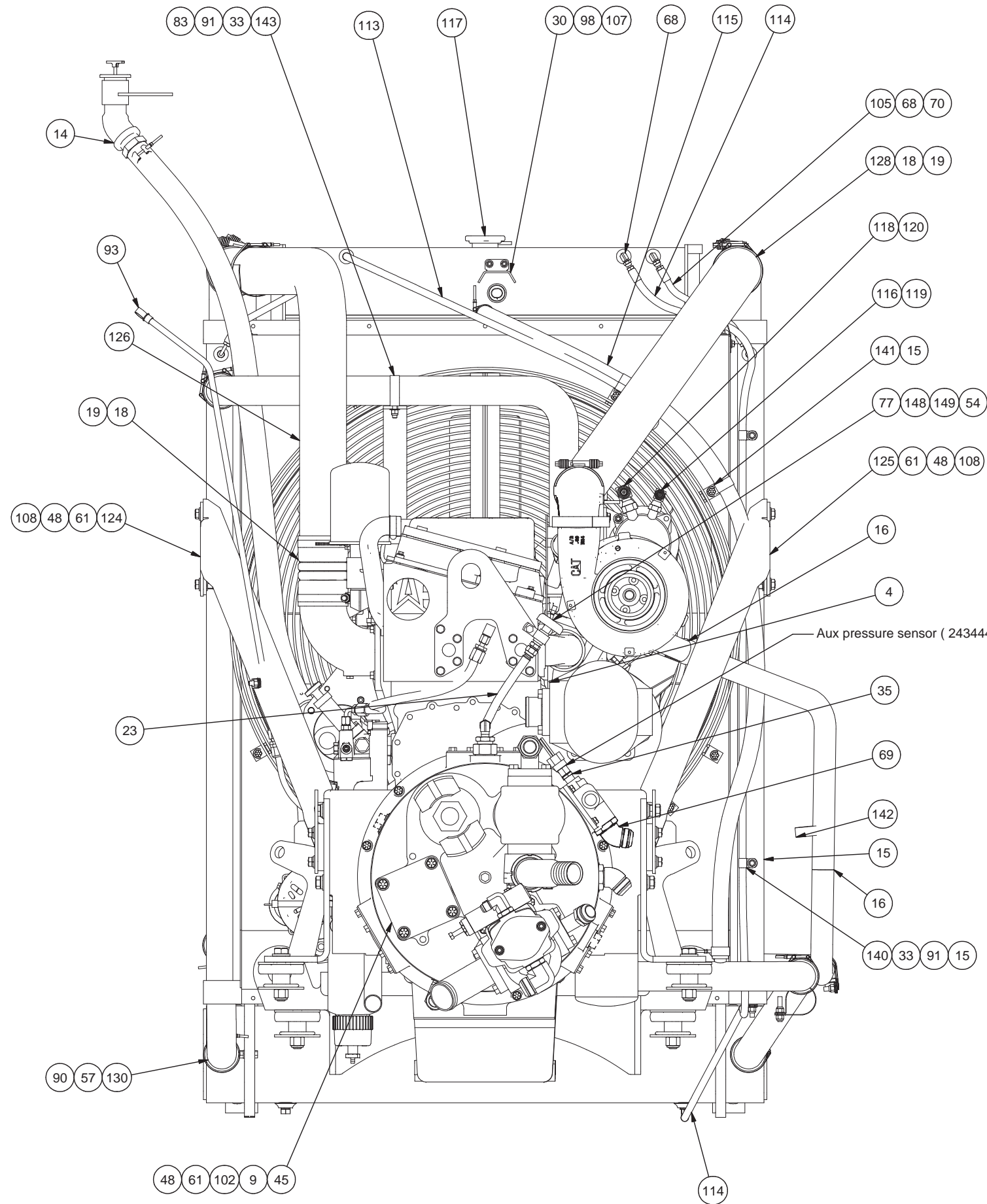
SECTION G-G
