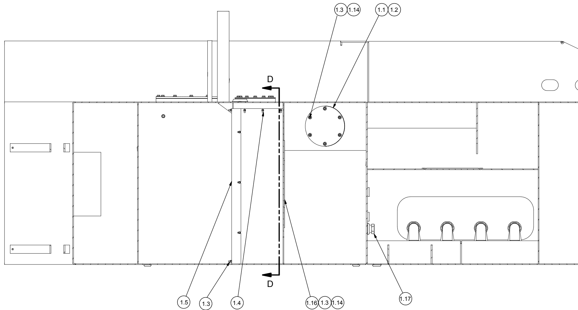
SECTION C-C
