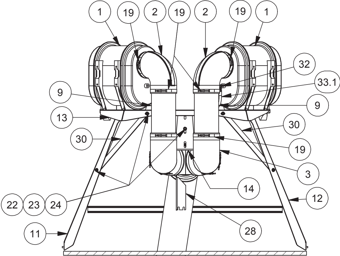
SECTION B-B
