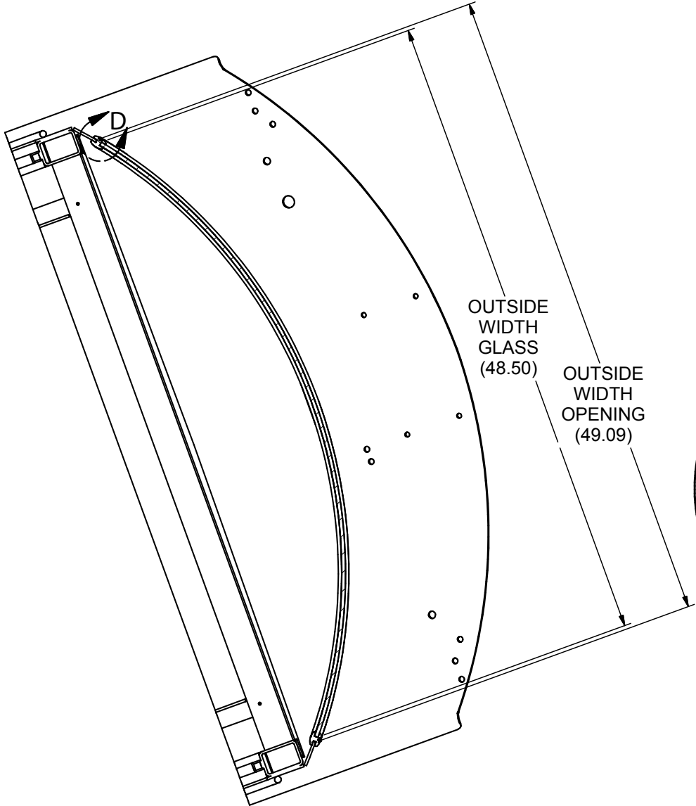
SECTION C-C
