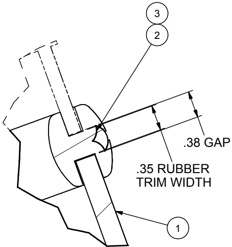
DETAIL B
