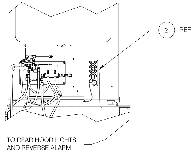
VIEW F-F
