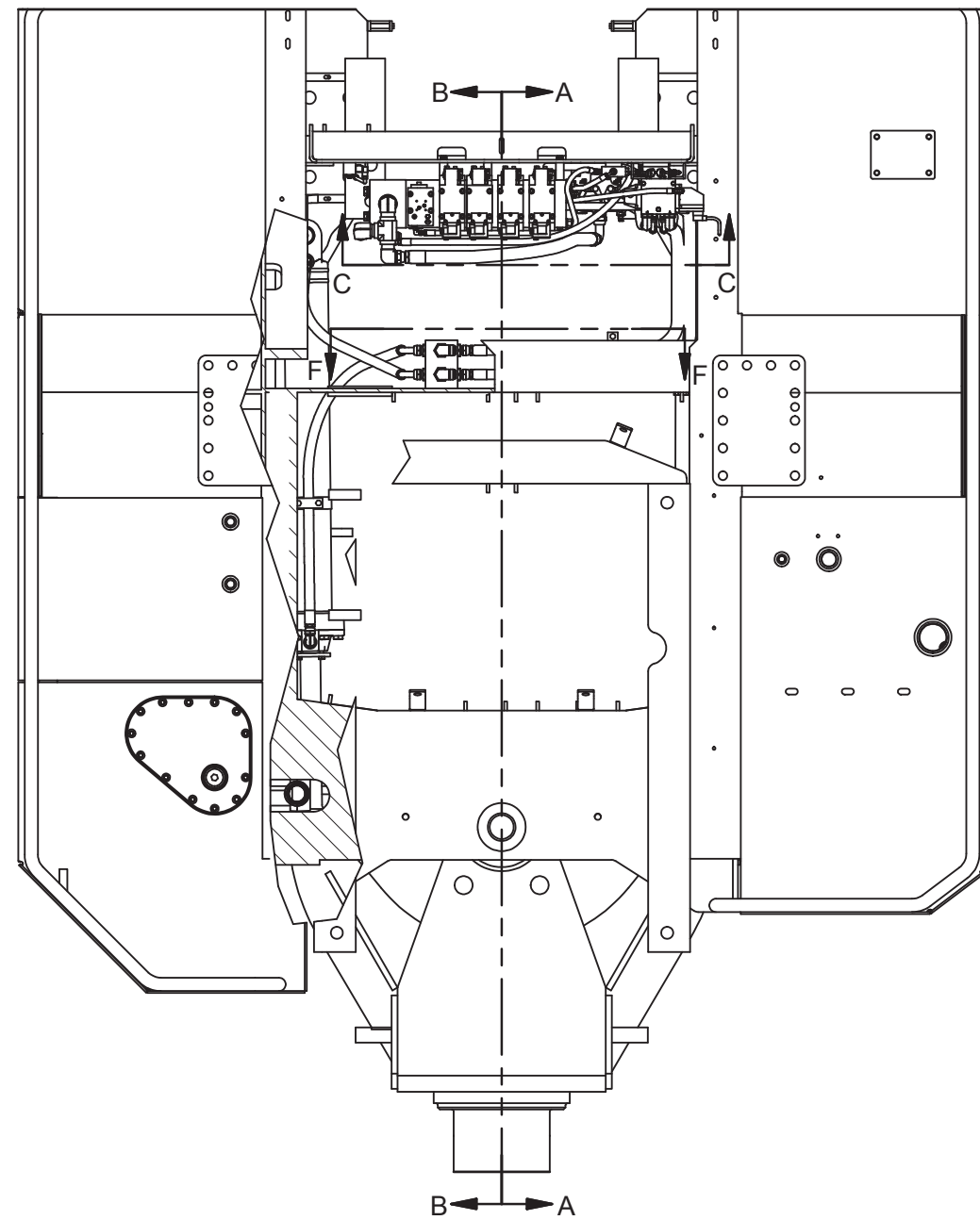
CHASSIS STEERING LAYOUT
