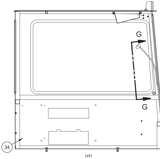
SECTION C-C JUNCTION BOX STUD LOCATION
