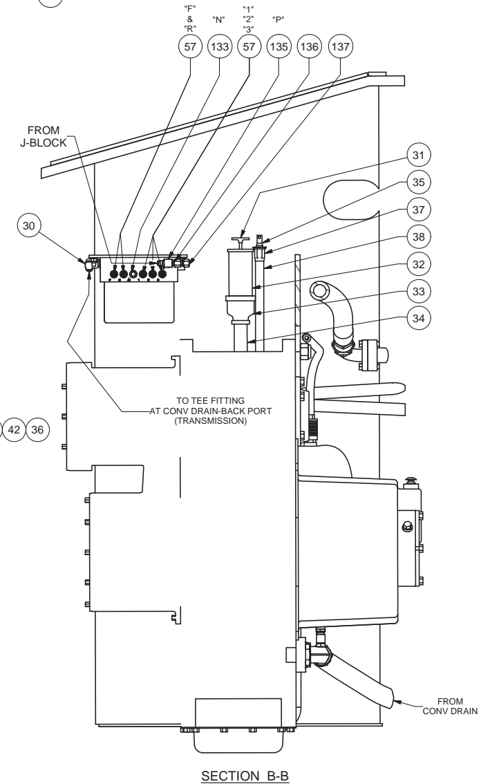
SECTION B-B
