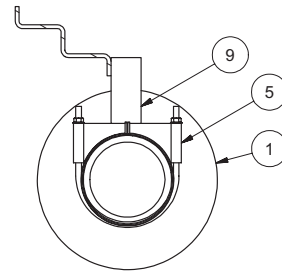
SECTION B-B TYPICAL (2 PLCS.)
