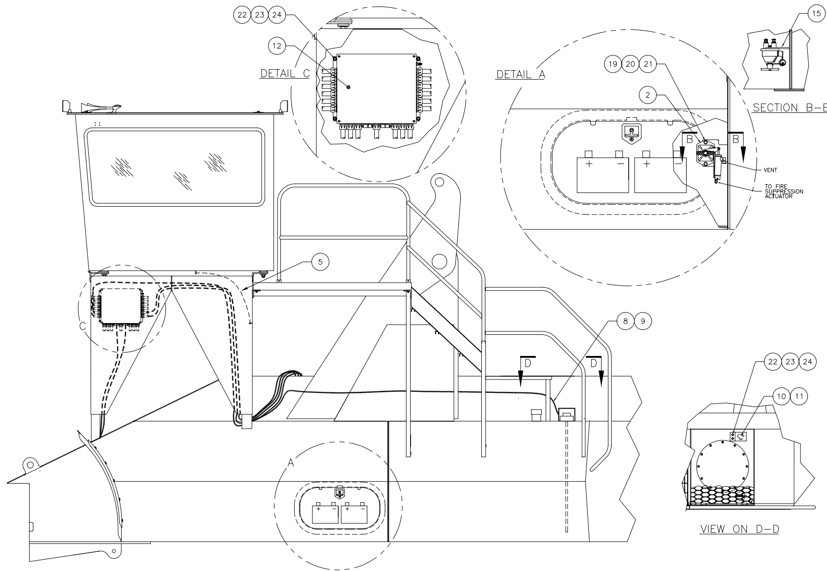
VIEW ON ENGINE, CHASSIS RH SIDE
