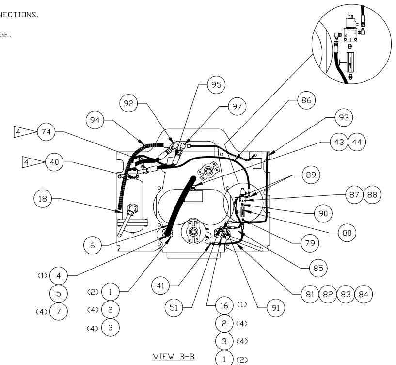
DETAIL A
