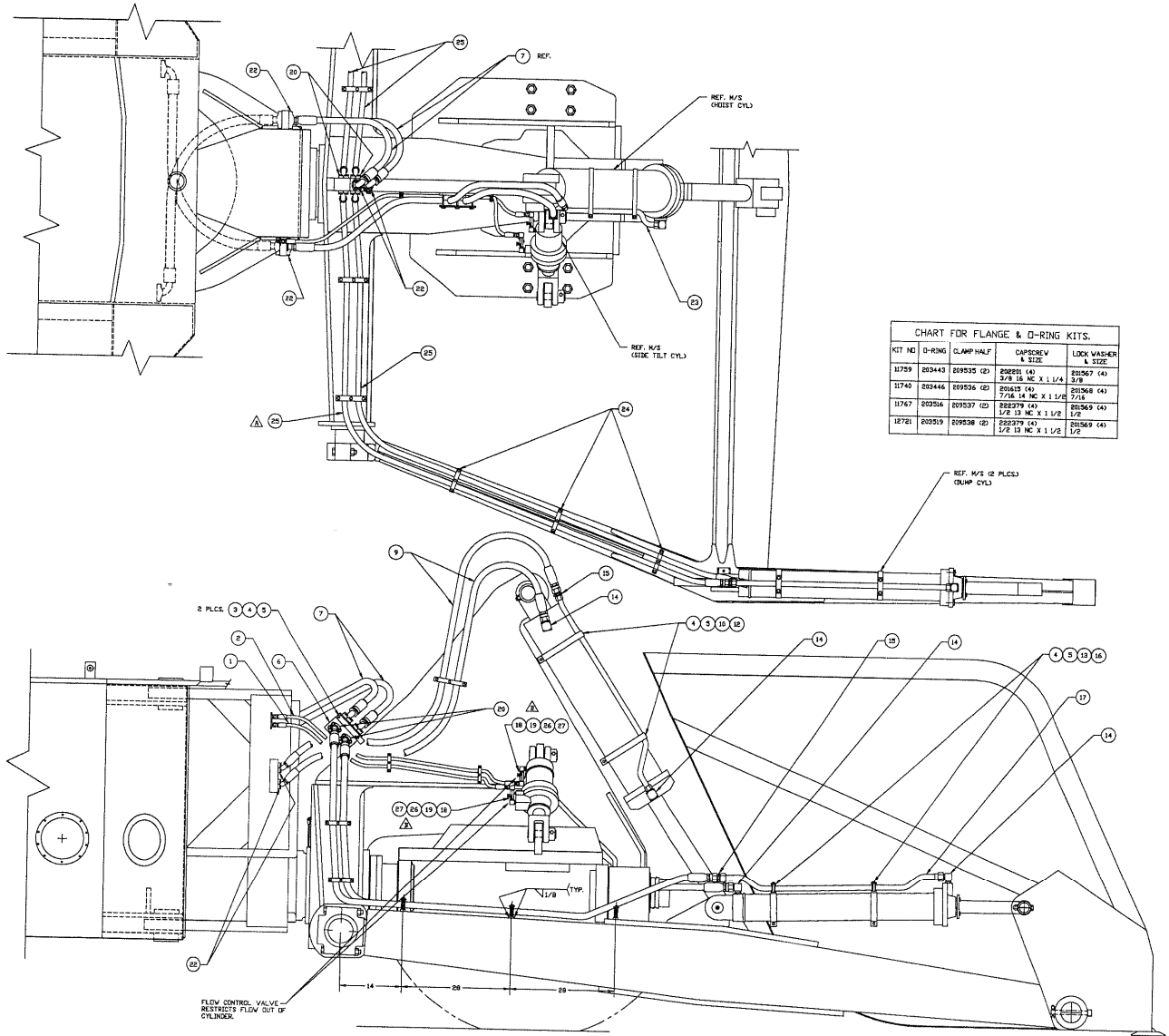
80 YD. BUCKET WITH SIDE TILT
