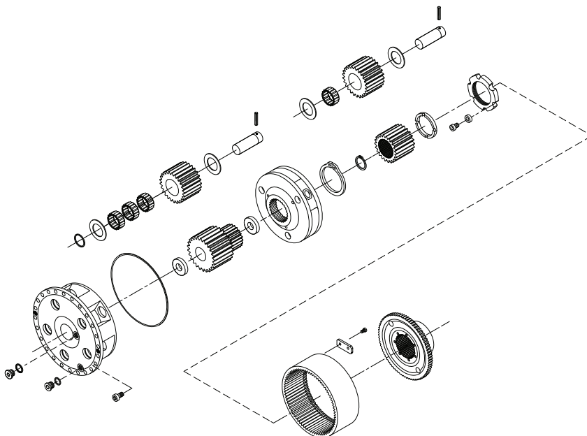
Figure 3-2-4 Planetary
