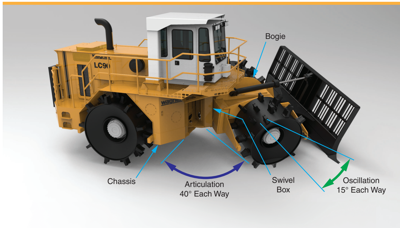
Figure 3-2-5 Chassis & Bogie
