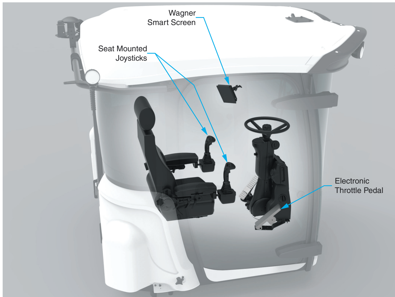
Figure 3-4-3 Operator Controls
