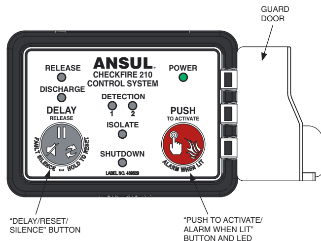
Figure 3-4-5 Checkfire 210 Detection and Actuation
