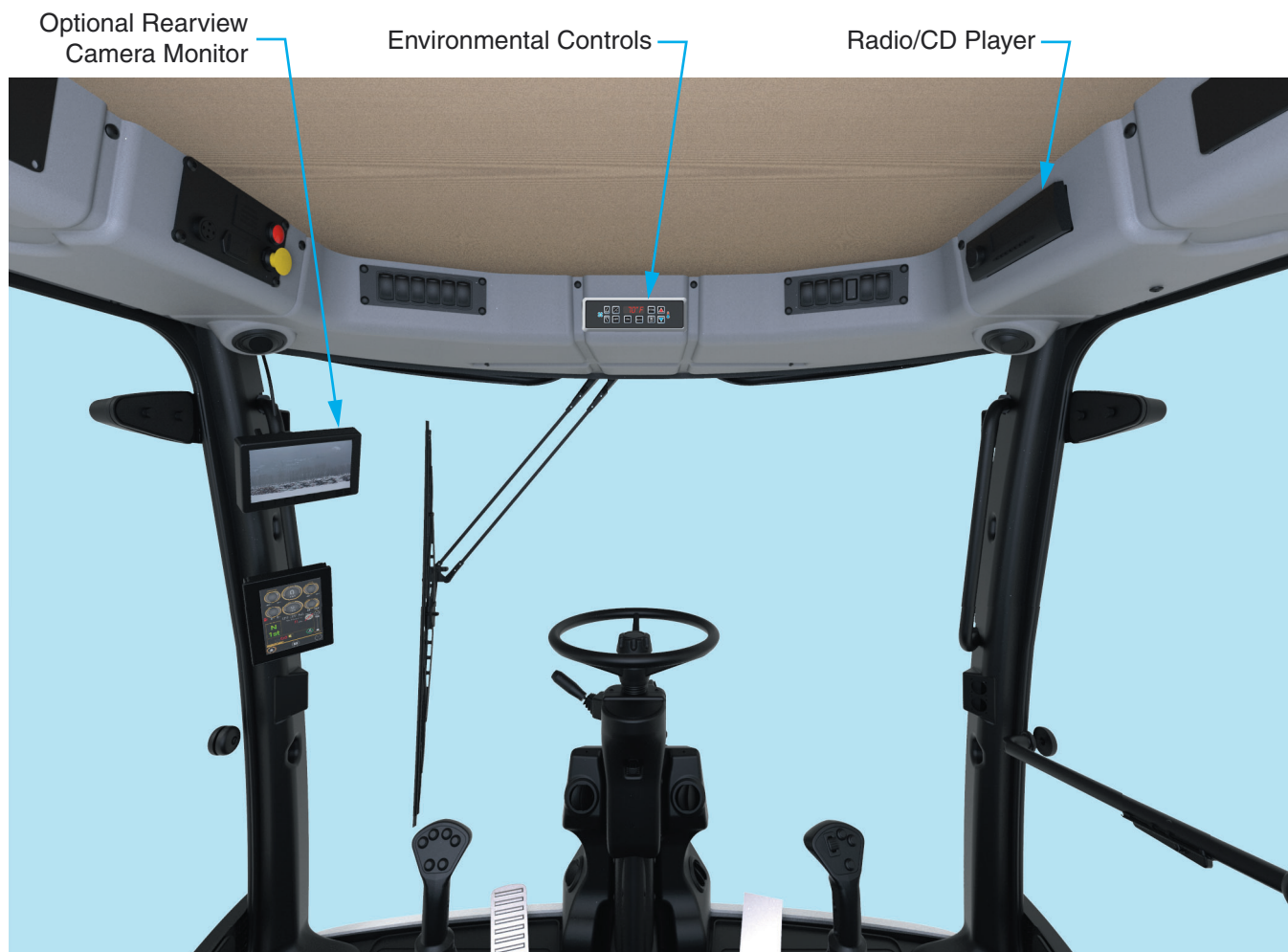
Figure 3-4-6 Environmental Controls and Rearview Camera Monitor
