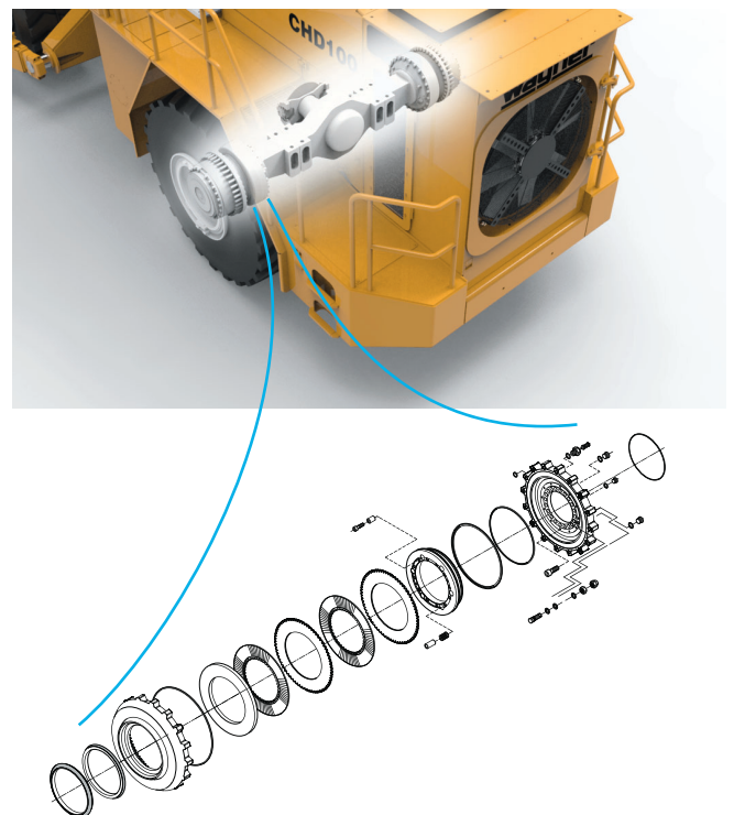
Figure 3-3-2 Wet Disc Brakes
