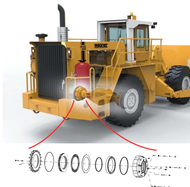
Figure 3-3-2 Wet Disc Brakes
