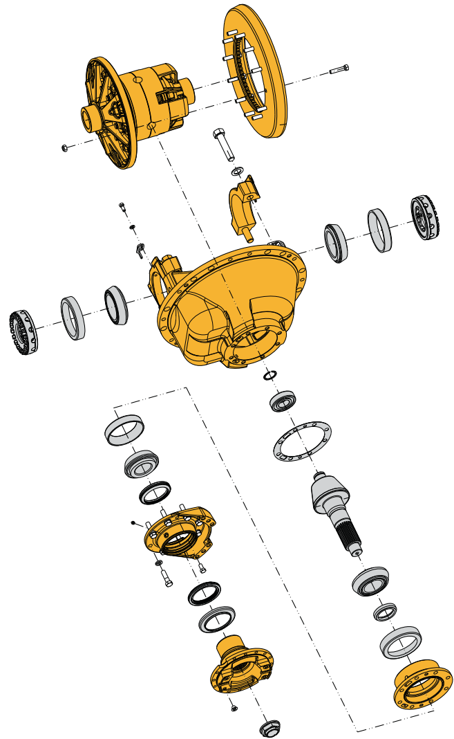
Figure 3-2-3 Differential
