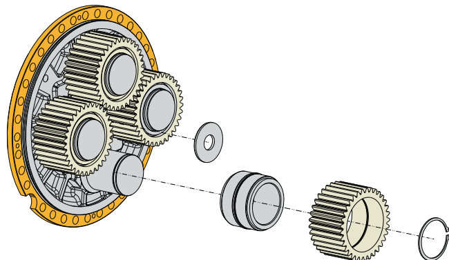
Figure 3-2-4 Planetary
