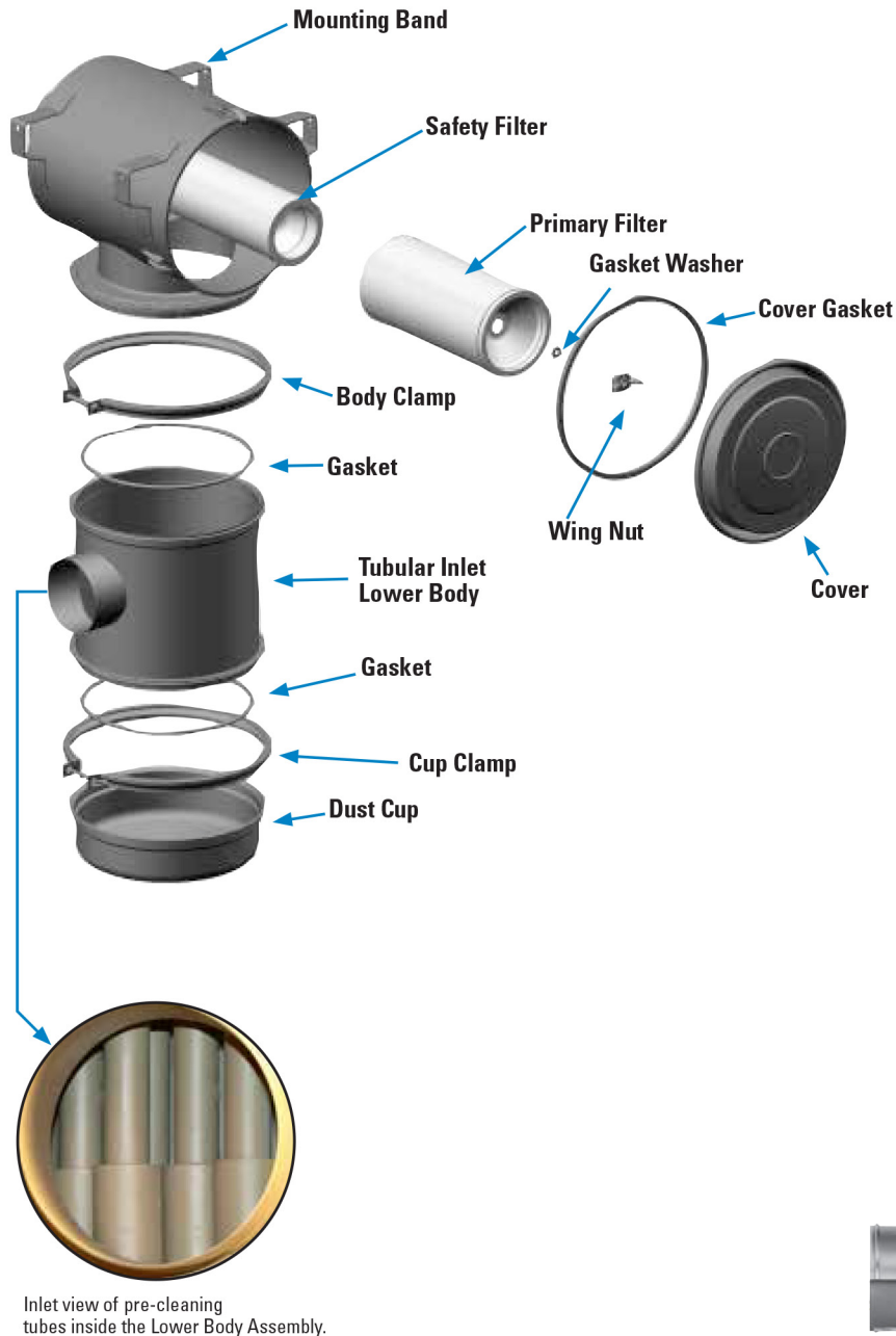
Figure 3-1-5 Air Cleaner Assembly
