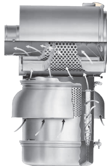
Figure 3-1-6 First Stage (Centrifugal Separation)
