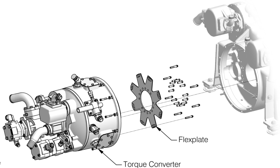
Figure 3-1-3 Torque Converter
