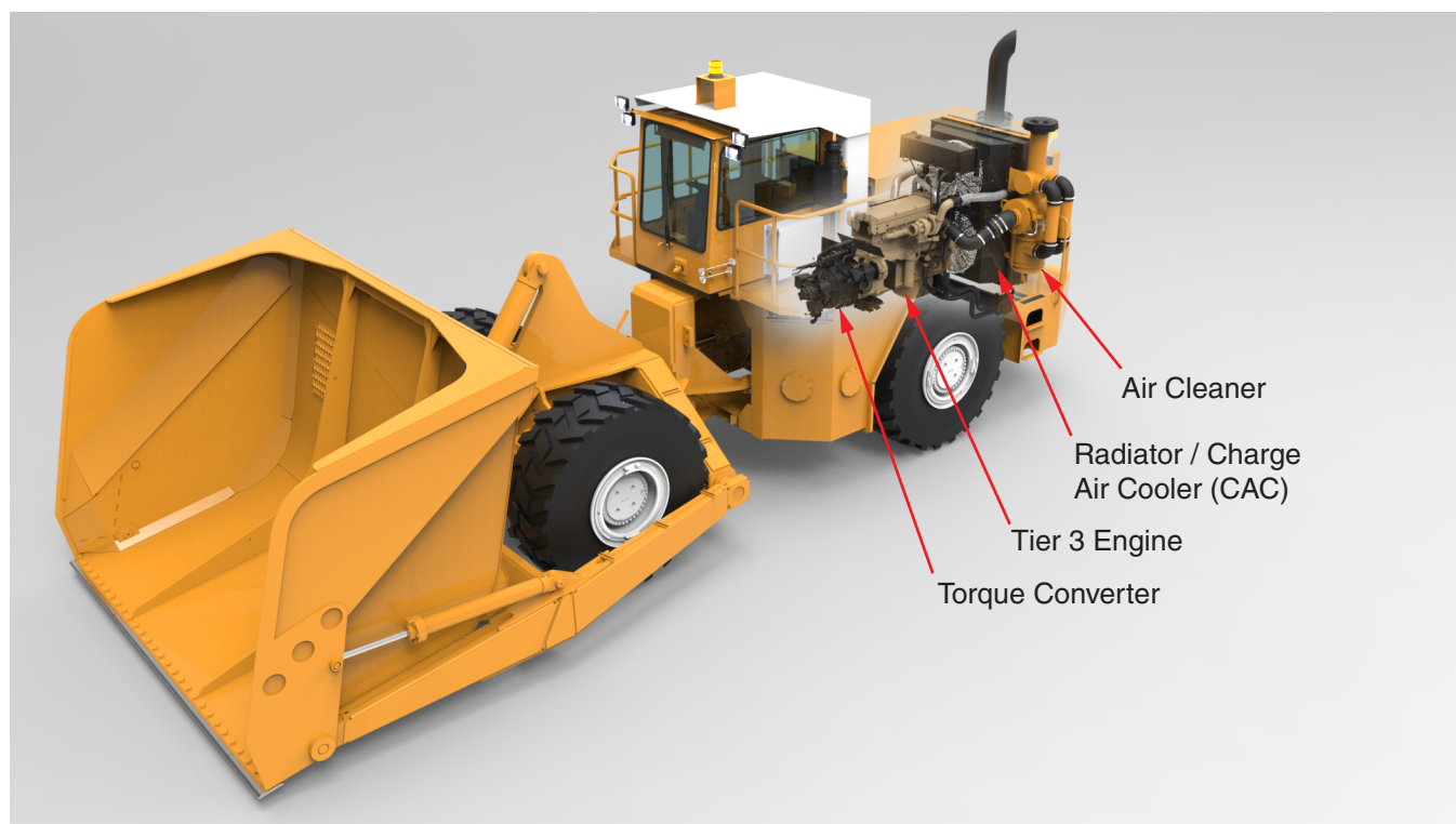
Figure 3-1-1 Power Unit (Model CHD100 with Tier 3 Engine Shown)
