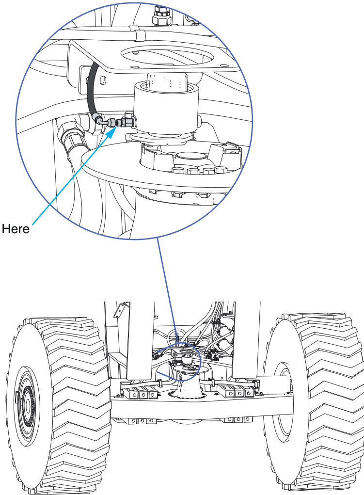
Figure 5-7-2 Connect Porta-Power
