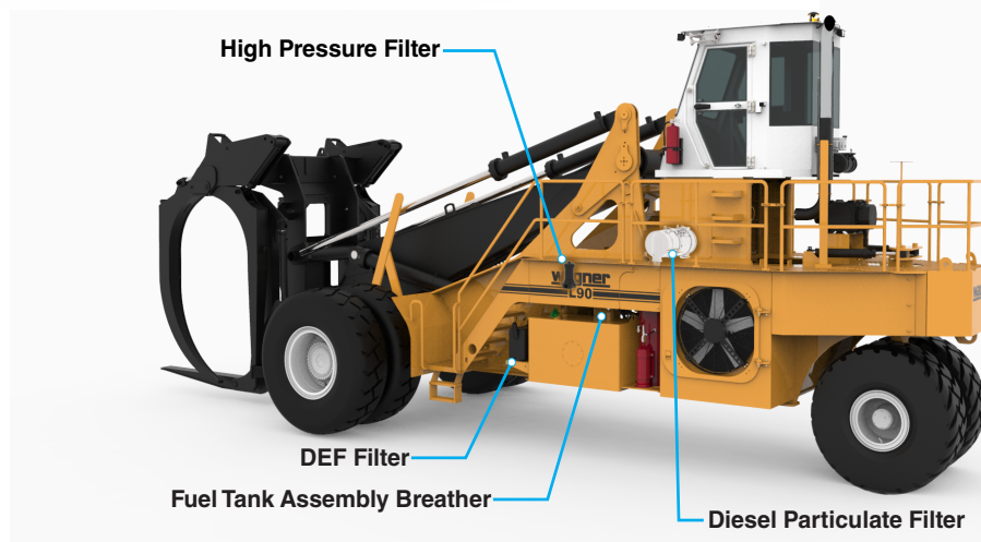
Figure 5-5-1 Filter Arrangement
