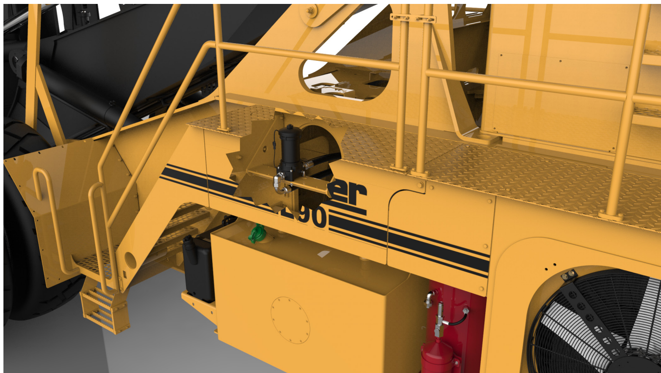
Figure 5-5-25 High Pressure Filter
