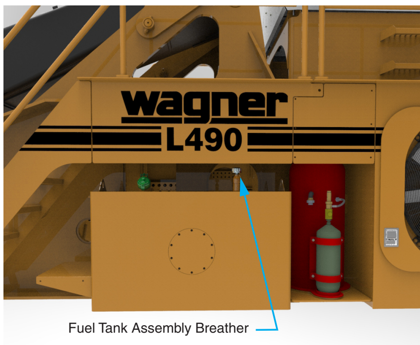
Figure 5-5-19 Fuel Tank Assembly Breather
