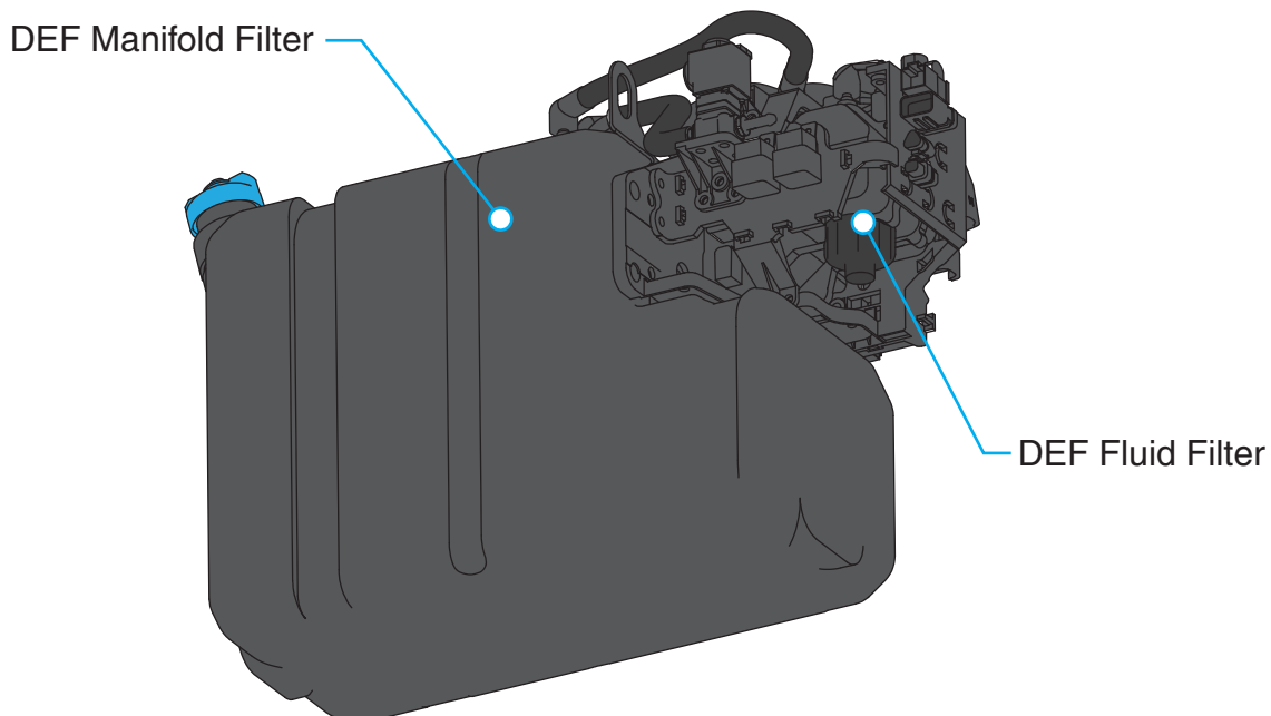
Figure 5-5-13 DEF Tank
