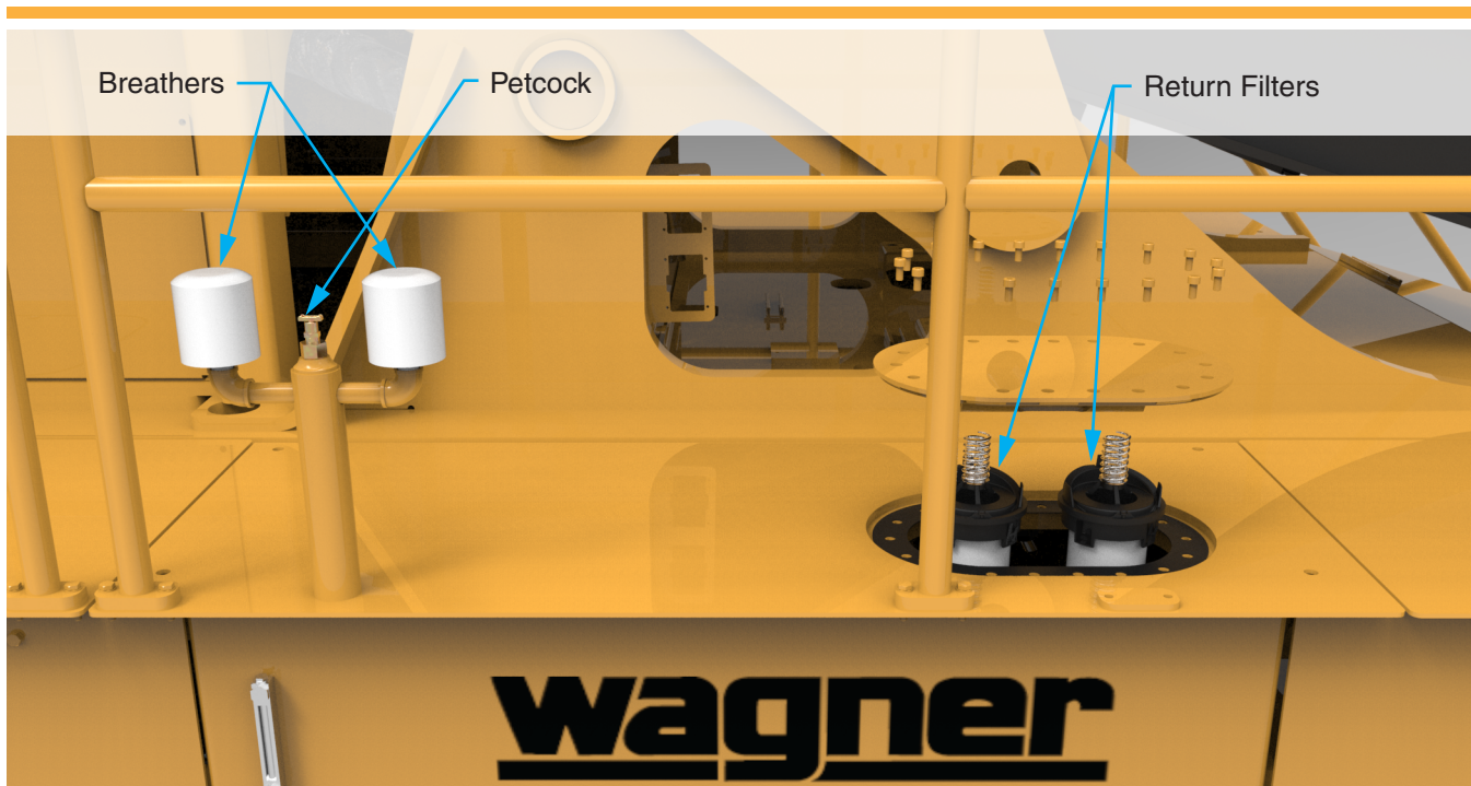
Figure 5-5-2 Return Filters
