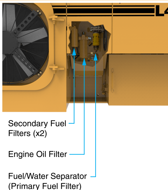
Figure 5-5-6 Engine Filters
