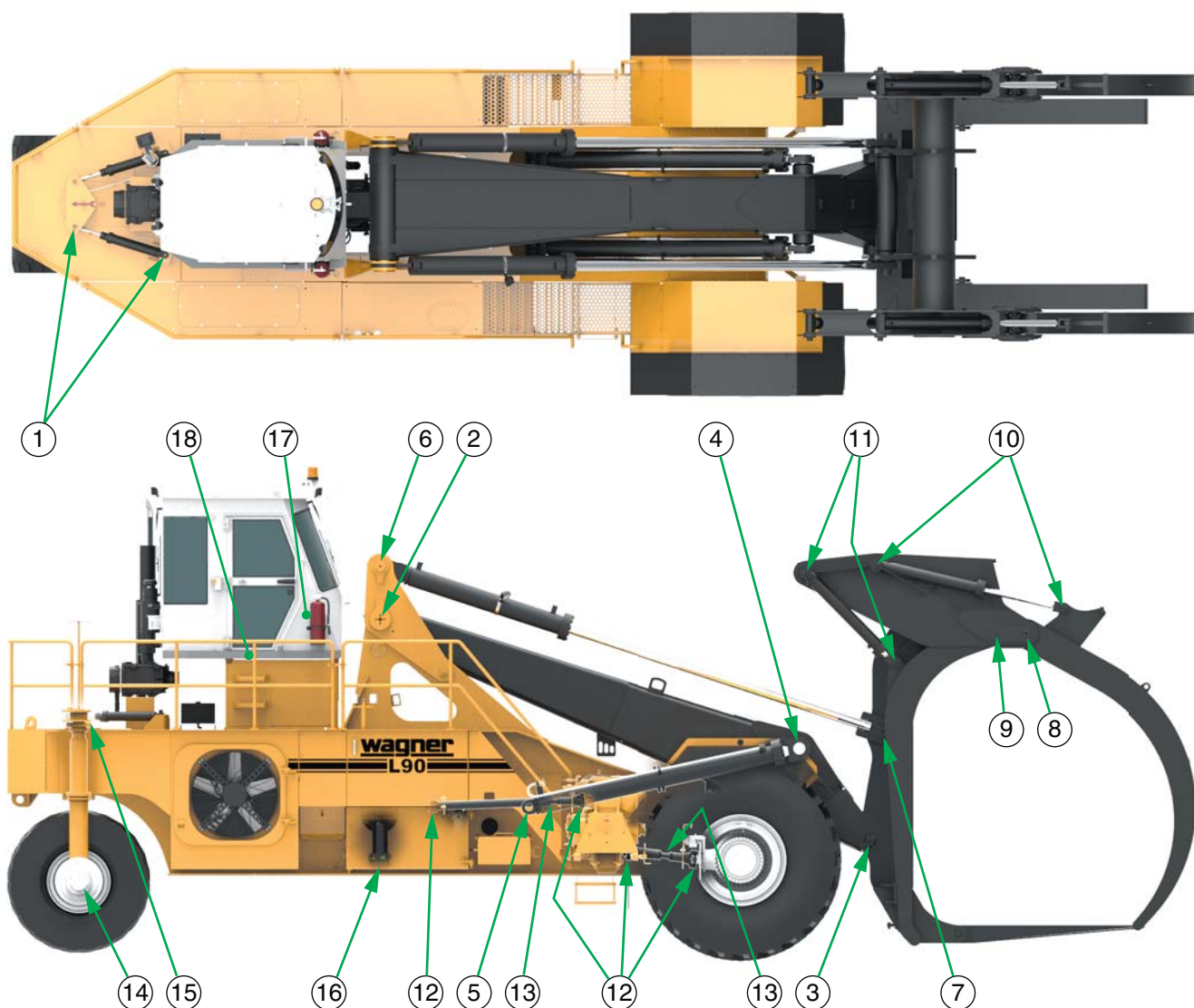
Figure 5-3-1 Lubrication Points
