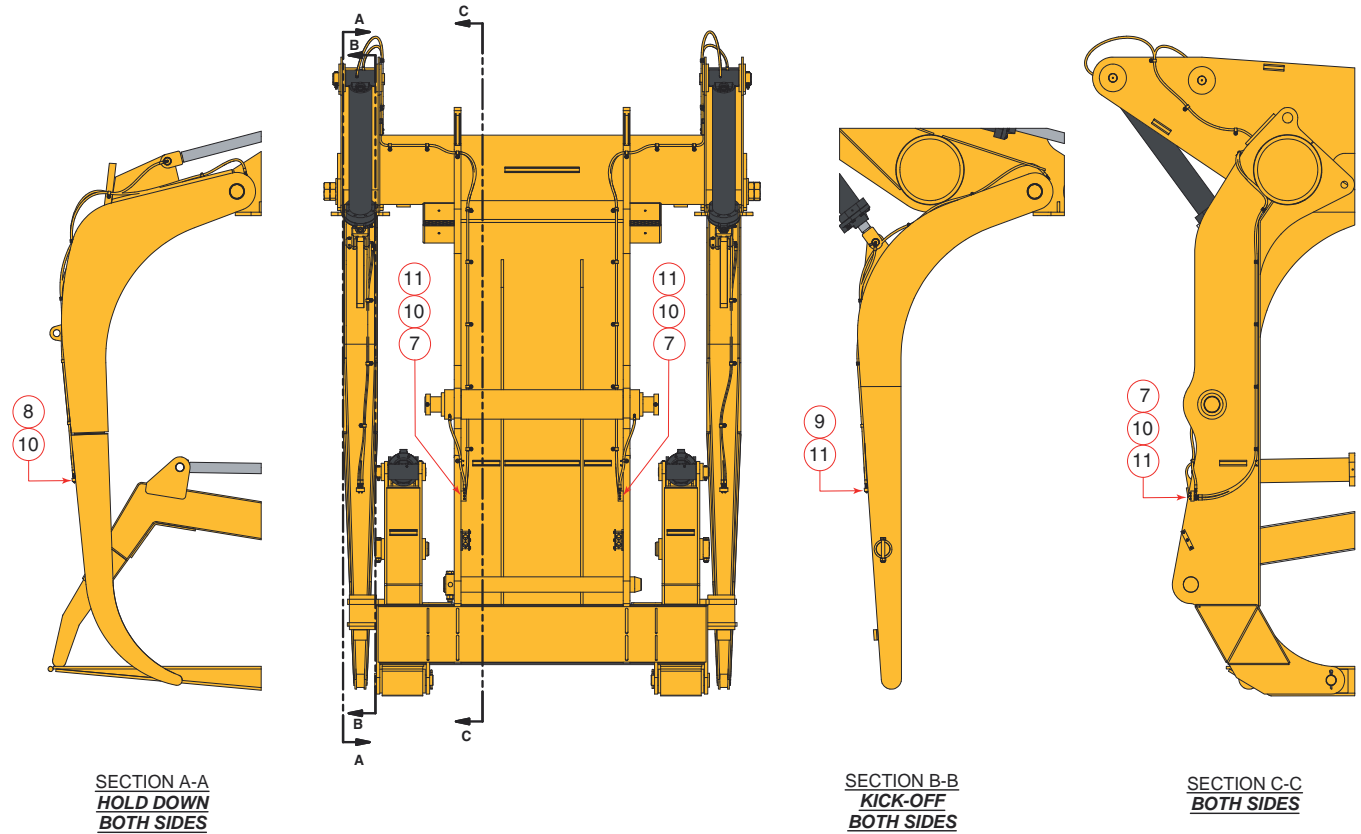
Figure 5-3-2 Remote Lube Fitting Locations
