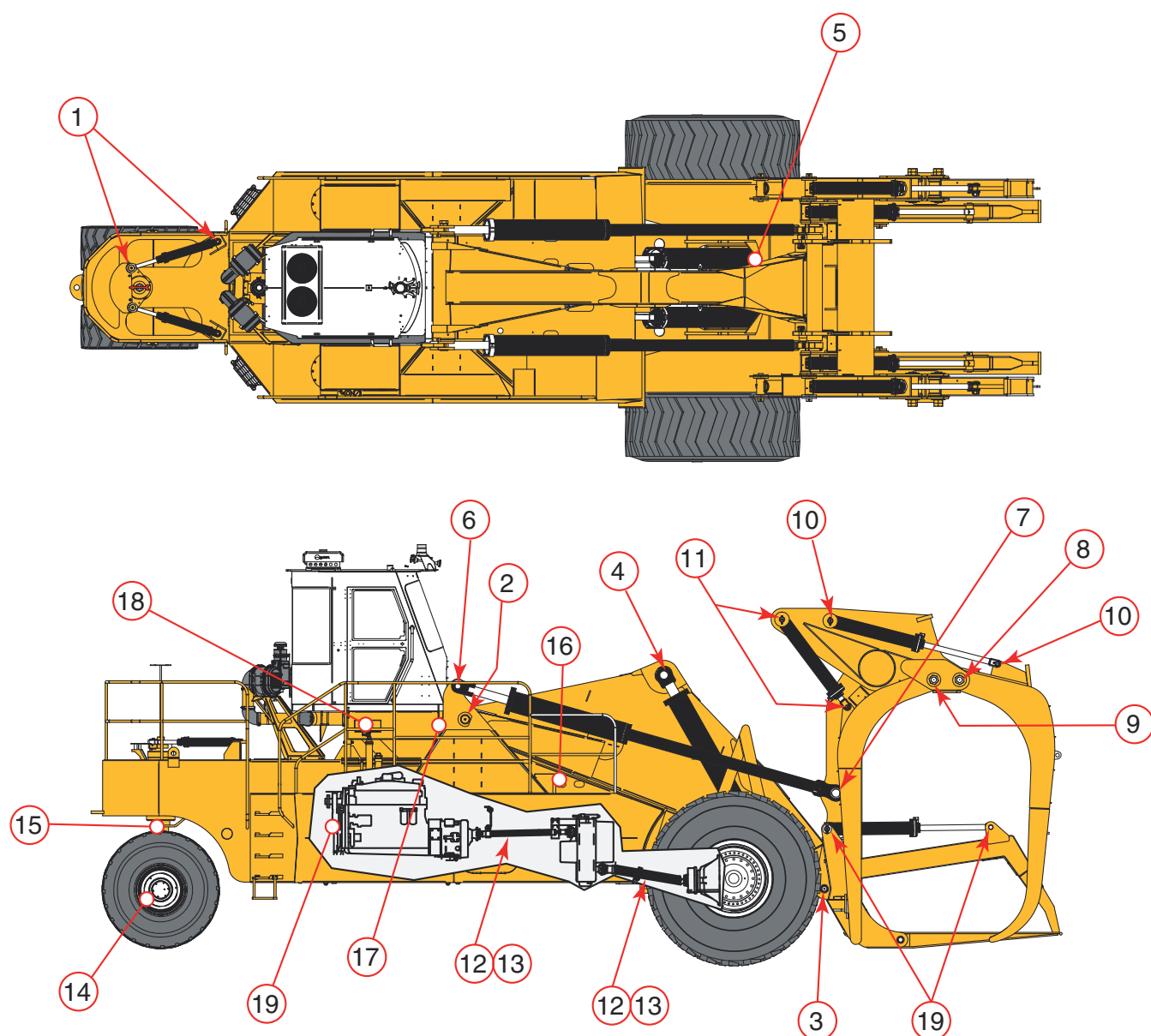
Figure 5-3-1 Lubrication Points
