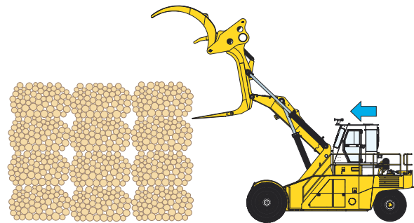
Figure 4-12-1 Approaching Deck
