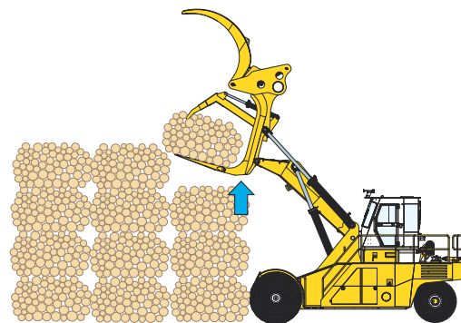
Figure 4-12-3 Lifting Bundle Off Stack
