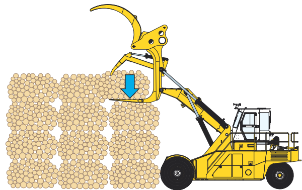
Figure 4-10-3 Flattening Lower Bundle Before Placing Top Bundle
