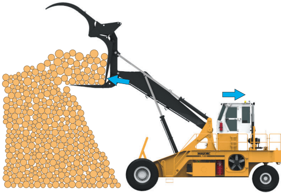
Figure 4-8-1 Adding Logs to the Top of a Stack
