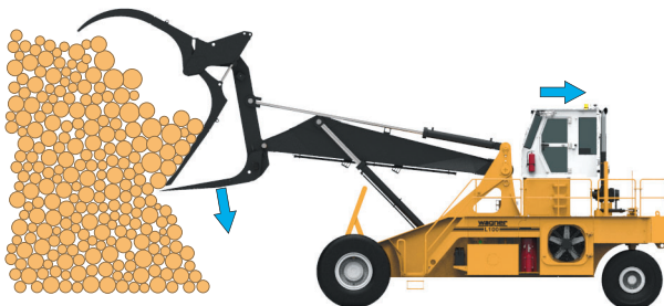
Figure 4-8-3 Backing Away to Empty the Carriage
