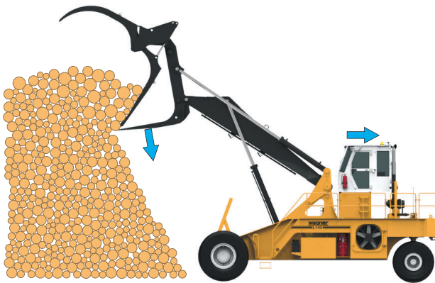
Figure 4-8-2 Adding Logs to the Front of the Stack
