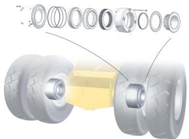
Figure 3-3-2 Wet Disc Brakes
