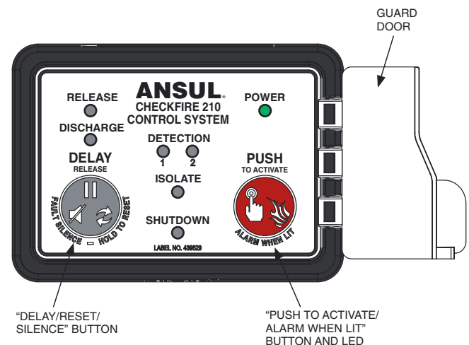
Figure 3-4-6 Checkfire 210 Detection and Actuation
