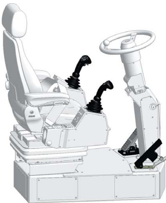
Figure 3-4-6 Operator Controls
