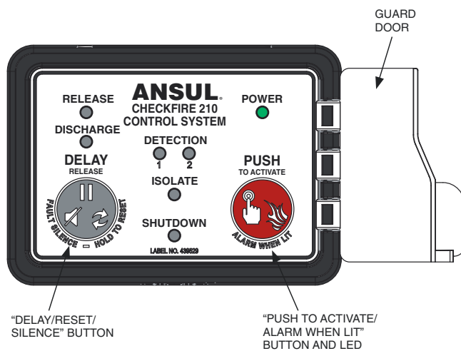
Figure 3-4-8 Checkfire 210 Detection and Actuation
