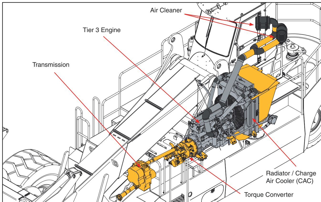
Figure 3-1-1 Power Unit (Model L90F with Cummins Tier 3 Engine Shown)
