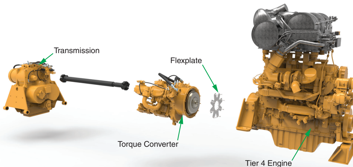
Figure 3-1-3 Torque Converter
