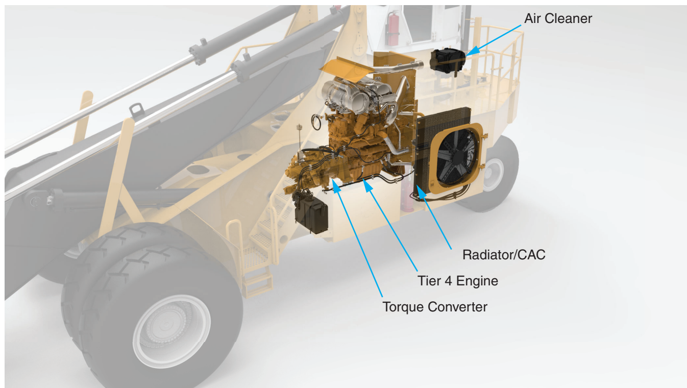
Figure 3-1-1 Power Unit (Model L100 with CAT Tier 4 Engine Shown)
