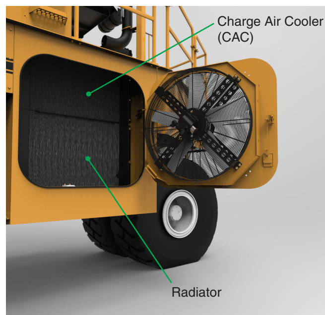
Figure 3-1-4 Cooling System
