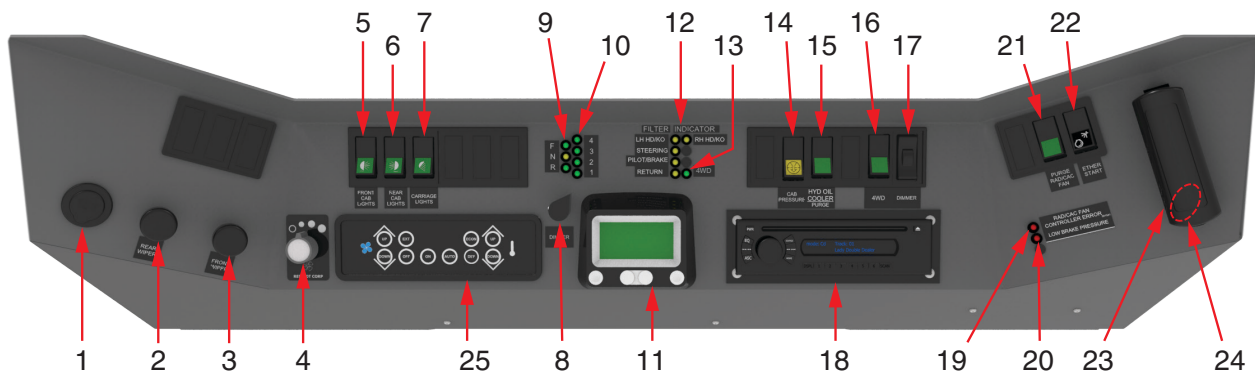
Figure 2-3-1 Overhead Console
